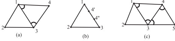
Fig. 5. Overall angularity is not necessarily generic. (a) Point 4 is unique when \{1, 3, 4\} are generic. (b) Point 4 is not unique when \{1, 3, 4\} are not generic. (c) \{2, 3, 5\} are not generic but angularity is rigid.
